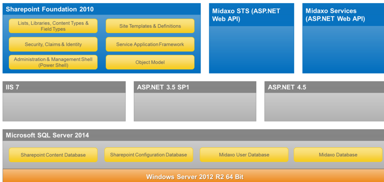
Figure 1 Software Architecture
